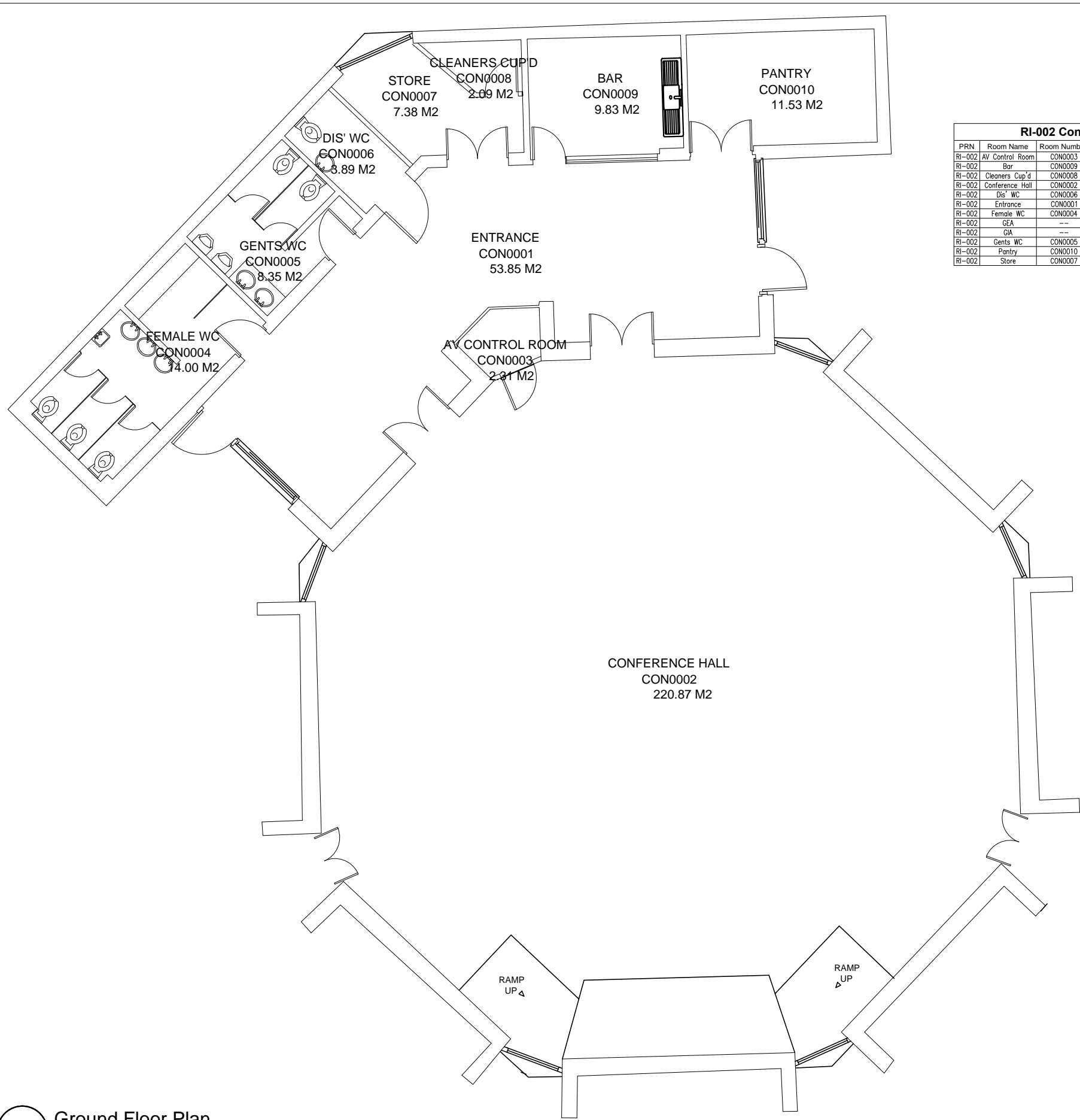
1000 Ground Floor Plan 1:100
